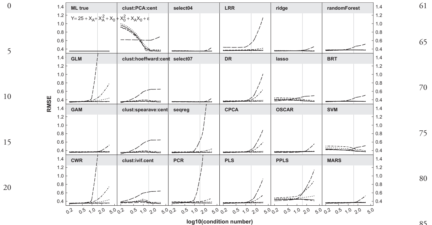
Figure 6. Relative prediction accuracy on test data for an ideal model (ML true) and 23 collinearity methods as a function of collinearity in the data set. In each panel, solid/short-hatched/dotted/dash-dotted/long-hatched locally-weighted smoothers (lowess) depict model predictions on same/more/less/non-linear/no correlation data sets accordingly (not discernable in function 5 for select07 and select04 because they yield nearly identical values). X-axis is \log(\text{condition number}) , depicted logarithmically. That is, x-values are in fact double-log-ed CNs (one log for the fact that CN is a ratio, the second because we chose logarithmic scaling of collinearity decay rates when generating the data). Data are scaled relative to simulated truth. an R^2 of 1 indicates as perfect prediction as possible. Vertical line (at CN = 30) indicates the rule-of-thumb threshold for CN beyond data set collinearity is deemed problematic.
