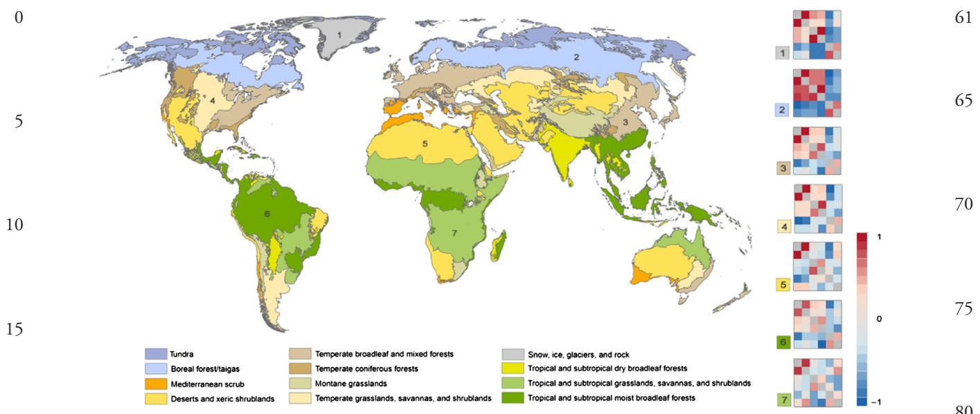
Figure 1. Changing collinearity structure of climate variables between eco-zones. Correlation matrix of the following six bioclimatic variables (< www.worldclim.org >): mean annual temperature, temperature seasonality (standard deviation), mean temperature of coldest quarter, annual precipitation, precipitation of driest month, precipitation seasonality (coefficient of variation). The upper triangular part of the matrix shows Pearson correlation coefficients, while the lower part shows Spearman coefficients. The diagonal elements are one by definition and displayed in grey.
