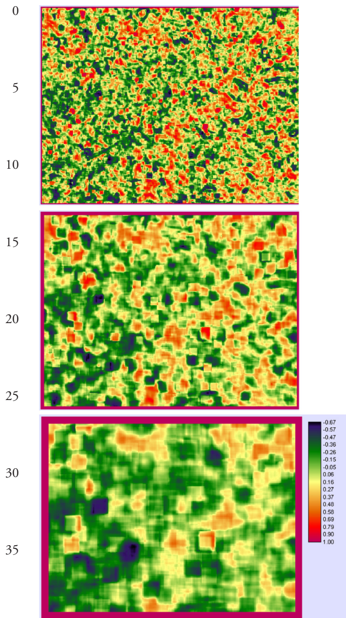
Figure 2. Correlations between environmental characteristics change with spatial resolution. Moving window Pearson correlations between principal components 1 and 2 of a Landsat TM scene for southern Portugal (pixel size 100 \times 100 m). Window size increases from 500 \times 500 m (top), through 1.1 \times 1.1 km (middle) to 2.1 \times 2.1 km (bottom). For the full image (i.e. a single window) the correlation is zero.
