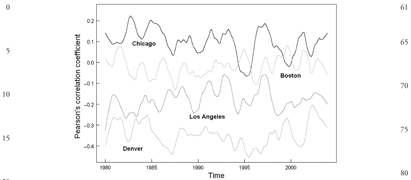
Figure 3. Smoothed time-series of the correlation between mean daily temperature and precipitation for four US-American cities. Systematic seasonal variation was removed by Loess decomposition (contributing about twice as much as the long-term trend depicted here). Moving window width is 30 d (data courtesy to Peter E. Thornton, Oak Ridge National Laboratories: < www.daymet.org >).
